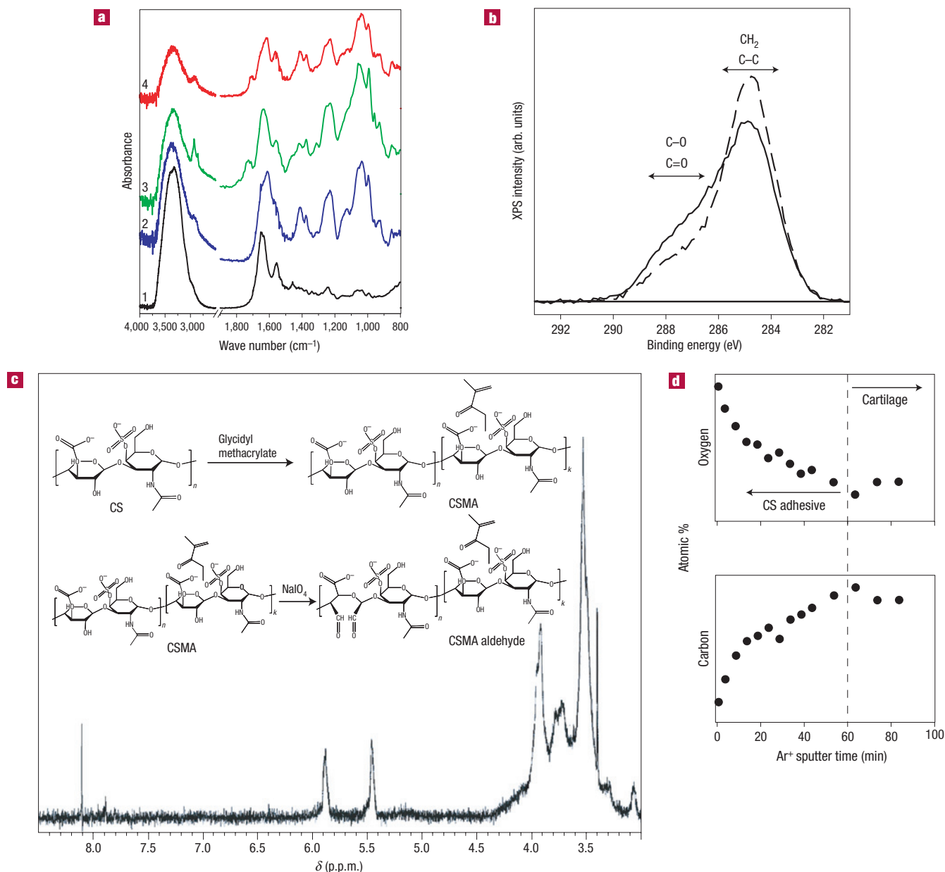
Figure 1 Synthesis and characterization of CS adhesive. a , ATR-FTIR spectra indicate the surface of unmodified native cartilage distinguished by stretching bands of protein amide-I at 1,640\text{ cm}^{-1} , amide-II at 1,550\text{ cm}^{-1} and amide-III at 1,240\text{ cm}^{-1} (spectrum 1); unmodified CS with stretching bands of saccharide alkyls at 2,920 , 2,850 and 1,415\text{ cm}^{-1} and alkoxyls at 1,030\text{ cm}^{-1} (spectrum 2); CS adhesive with stretching bands of carbonyl at 1,730\text{ cm}^{-1} (spectrum 3); and CS adhesive on the cartilage surface, which contains peaks from both cartilage and the functionalized CS (spectrum 4). b , The C(1s) XPS regions of untreated cartilage (dashed line) and cartilage treated with CS adhesive (solid line) exhibit different concentrations of oxygen containing carbon functional groups at the surface. This supports the idea that the CS adhesive is present on the tissue surface. c , ^1\text{H} NMR analysis: alkyl protons on saccharide backbone at a chemical shift \delta 3.2 \sim 4.0 p.p.m.; vinyl protons on methacrylate at \delta 5.89 and 5.44 p.p.m.; aldehyde protons at \delta 8.11 p.p.m. Inset: CS-adhesive synthesis pathway. d , Depth profile for a cartilage surface treated with CS adhesive. The tissue was sputtered with \text{Ar}^+ and the variation in the carbon and oxygen content at the surface was measured using XPS. The oxygen and carbon concentration changed over the initial 60 min of sputter time, after which the chemical composition of the surface remained constant, indicating that all of the adhesive had been removed from the cartilage surface.
